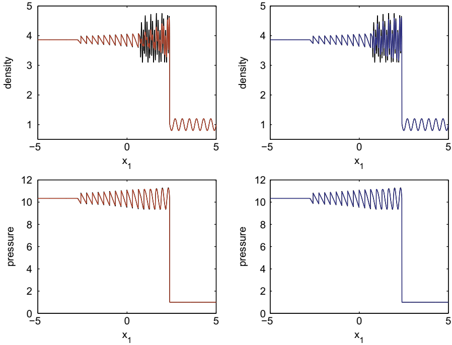
Fig. 7. Comparison of the numerical approximations at t = 1.8 for the Shu–Osher test problem and m = 16 . For all images the black line represents the reference solution with m = 128 while the red line (left) shows the Godunov approximation and the blue line (right) shows the FCT approximation. From top to bottom are density and pressure. (For interpretation of the references to colour in this figure legend, the reader is referred to the web version of this article.)
