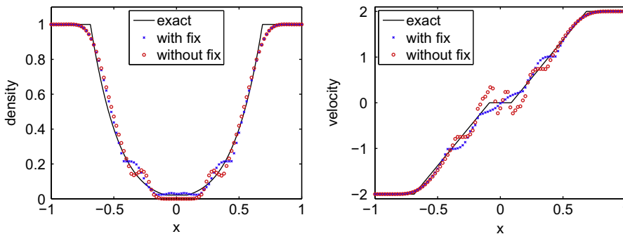
Fig. 2. Density (left) and velocity (right) for a strong rarefaction problem at t = 0.25 . The black line represents the exact solution, the red circles the FCT approximation without a fix and the blue crosses the FCT solution with the fix. The oscillations in velocity for the original FCT scheme are particularly troubling but also note the undershoot of the density near the origin. (For interpretation of the references to colour in this figure legend, the reader is referred to the web version of this article.)
