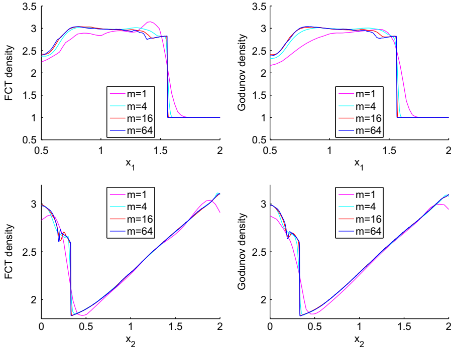
Fig. 12. Solution convergence along the lines x_2 = 0 (top) and x_1 = 1 (bottom) for the FCT method (left) and the Godunov method (right) on the shock-cylinder problem. Shown here is the density with the colors indicating numerical resolution. Maroon represents the solution with no AMR while cyan, red, and finally blue represent 1, 2, and 3 levels of additional factor four adaptive meshes, respectively. (For interpretation of the references to then, red,
