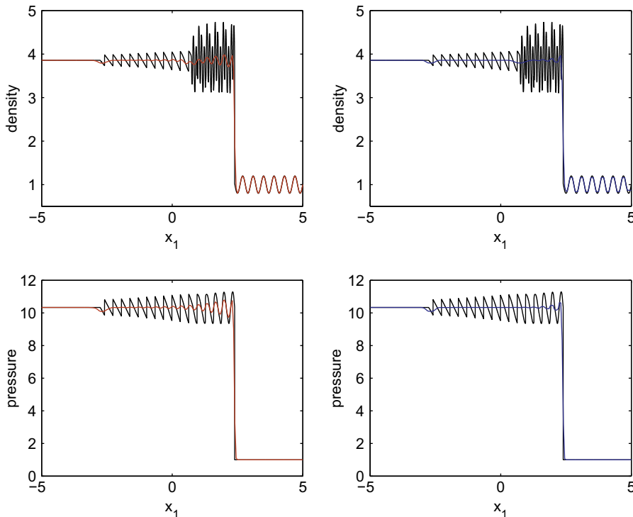
Fig. 5. Comparison of the numerical approximations with m = 1 at t = 1.8 for the Shu–Osher test problem. For all images the black line represents the reference solution with m = 128 while the red line (left) shows the Godunov approximation and the blue line (right) shows the FCT approximation. From top to bottom are density and pressure. (For interpretation of the references to colour in this figure legend, the reader is referred to the web version of this article.)
