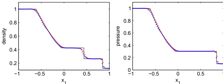
Fig. 3. Exact solution (black line) and numerical approximations with m = 1 for Godunov's method using Roe's approximate Riemann solver (red marks) and the FCT method (blue marks) for the modified Sod shock tube problem at t_f = 0.5 . Shown here are the density (left) and the pressure (right). (For interpretation of the references to colour in this figure legend, the reader is referred to the web version of this article.)
